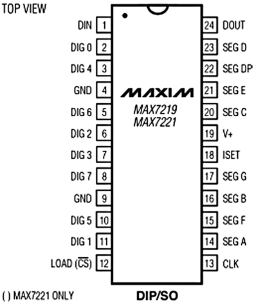
Figure 7-5. Pin diagram for the MAX7219
